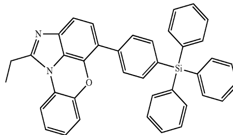
[Chemical Formula 1-9-13]
