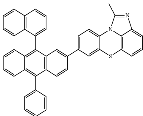
[Chemical Formula 2-2-22]
