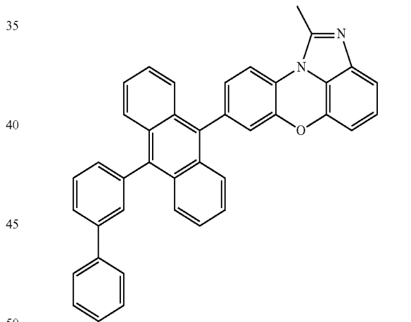
[Chemical Formula 1-2-7]
