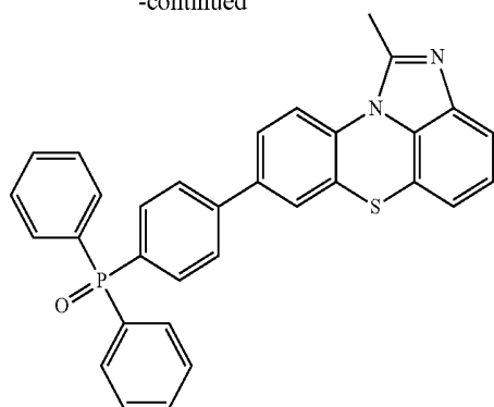
[Chemical Formula 2-4-1]
