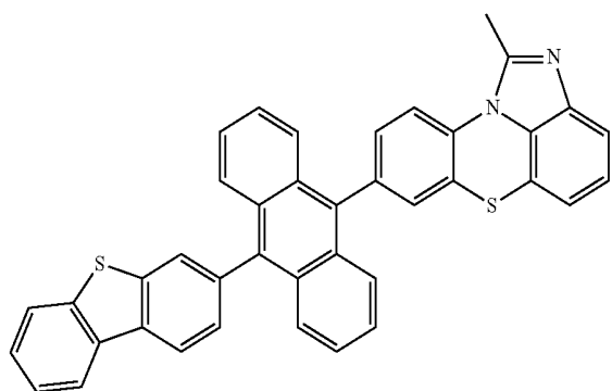
[Chemical Formula 2-2-14]
