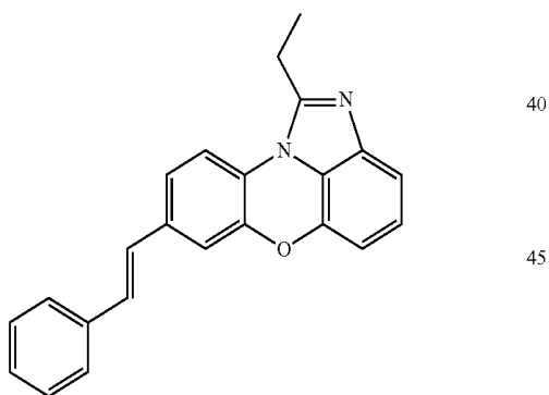
[Chemical Formula 1-4-1]
