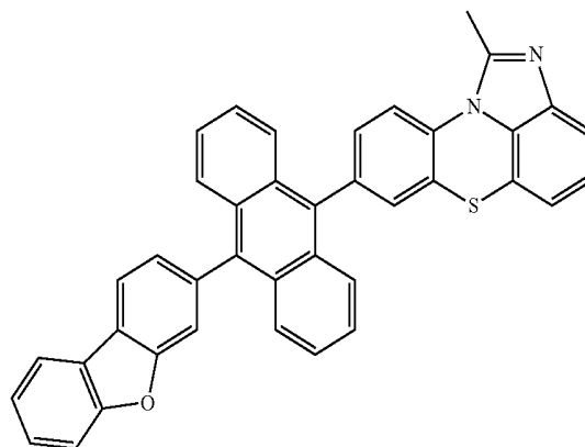
[Chemical Formula 2-2-14]
