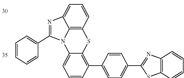
[Chemical Formula 2-2-47]
