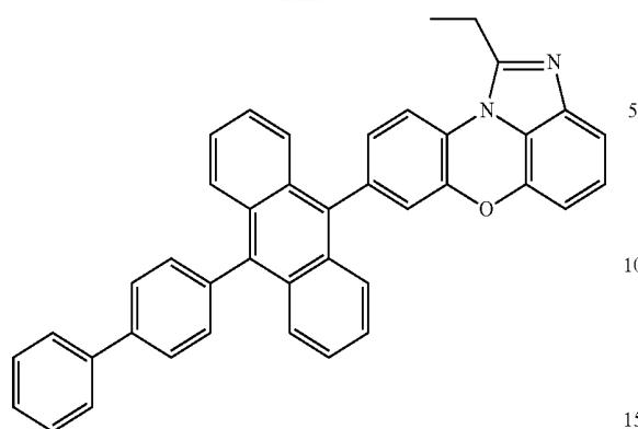
[Chemical Formula 1-3-4]
