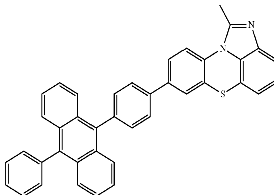
[Chemical Formula 2-2-18]
