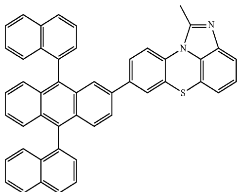
[Chemical Formula 2-2-21]
