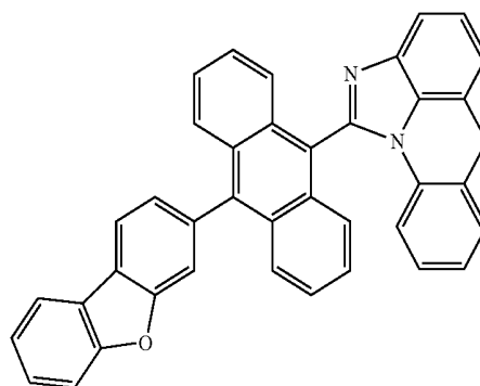
[Chemical Formula 1-1-21]
