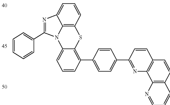
[Chemical Formula 2-2-48]
