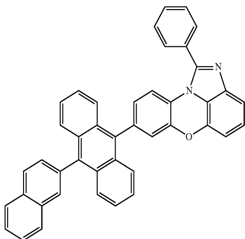
[Chemical Formula 1-4-2]
