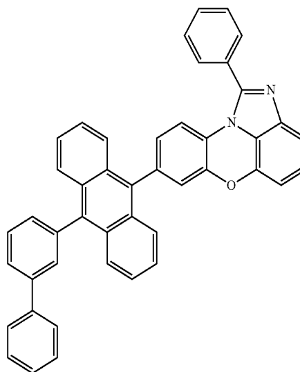
[Chemical Formula 1-4-6]
