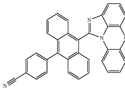
[Chemical Formula 1-1-21]
