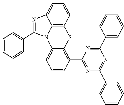
[Chemical Formula 2-2-41]
