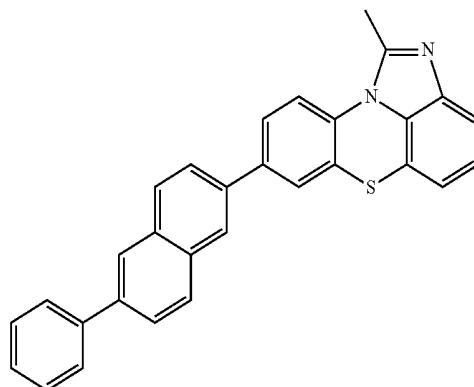
[Chemical Formula 2-2-27]
