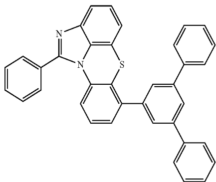
[Chemical Formula 2-2-40]
