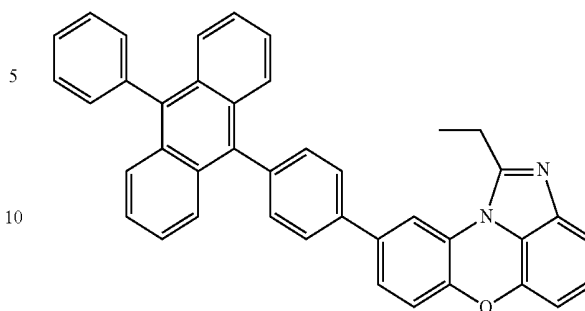
[Chemical Formula 1-7-17]
