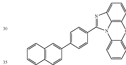
[Chemical Formula 1-1-34]
