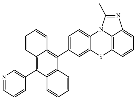
[Chemical Formula 2-2-10]
