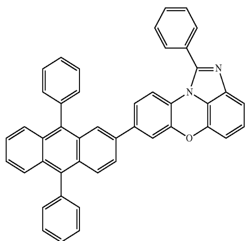
[Chemical Formula 1-4-19]
