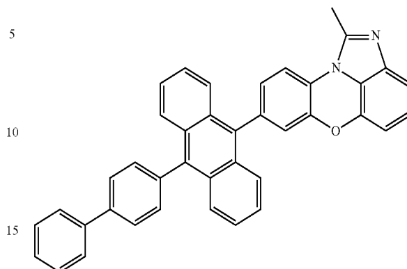
[Chemical Formula 1-2-5]
