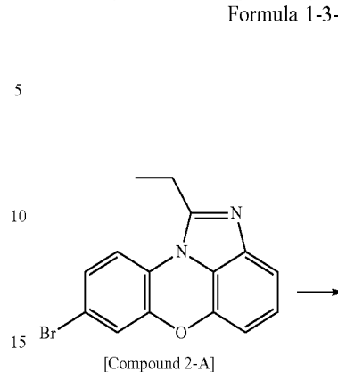
[Compound 2-A]
