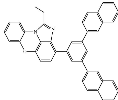
[Chemical Formula 1-11-8]
