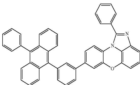
[Chemical Formula 1-4-18]
