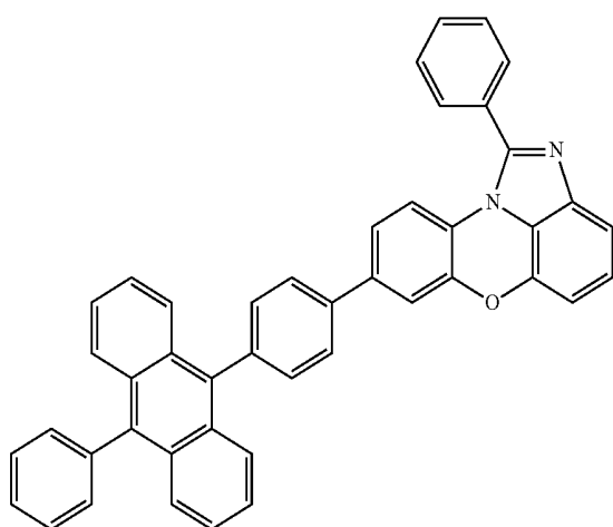
[Chemical Formula 1-4-17]
