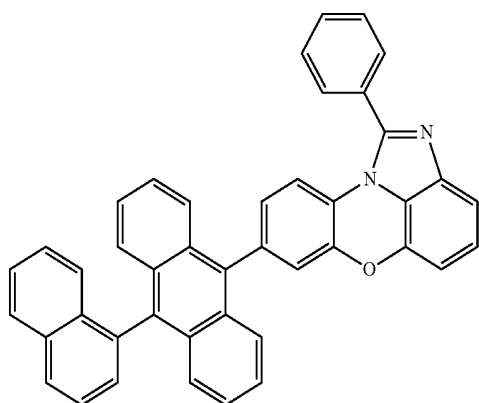
[Chemical Formula 1-4-3]
