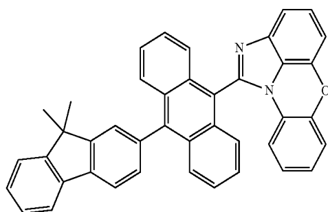
[Chemical Formula 1-1-13]
