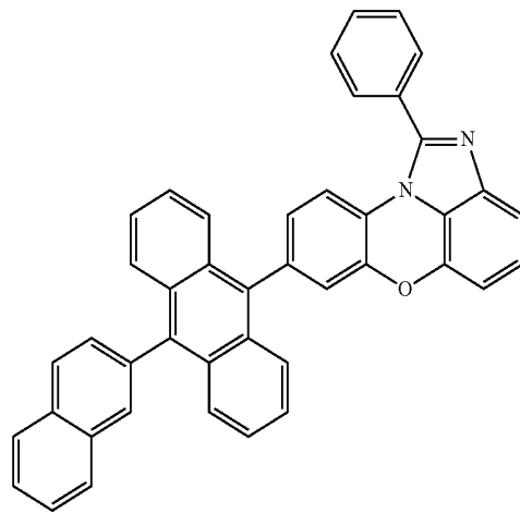
[Chemical Formula 1-4-2]
