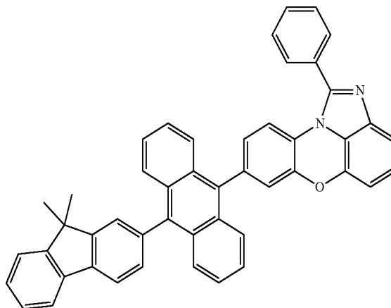
[Chemical Formula 1-4-5]
