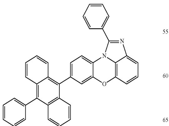
[Chemical Formula 1-4-1]
