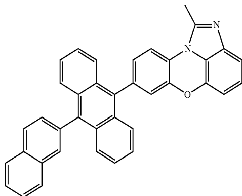
[Chemical Formula 1-2-3]
