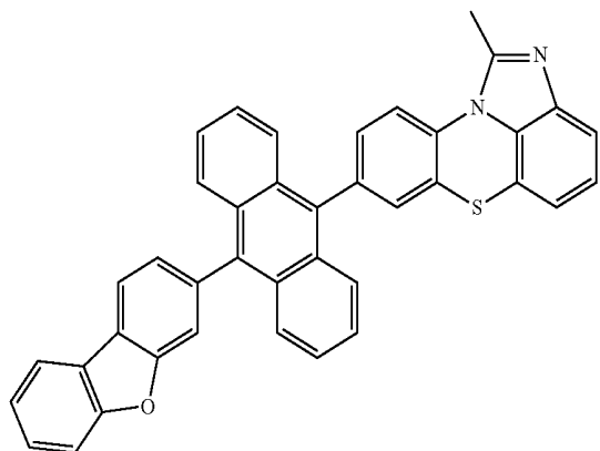
[Chemical Formula 2-2-14]
