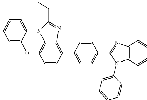
[Chemical Formula 1-11-10]
