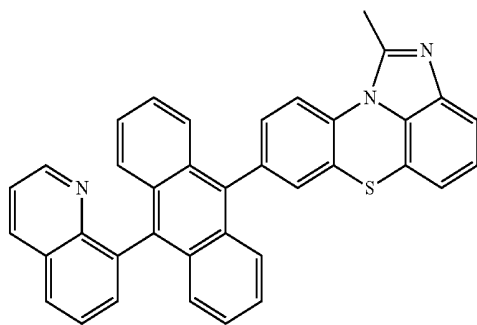
[Chemical Formula 2-2-11]
