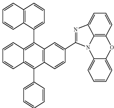
[Chemical Formula 1-1-30] 5
