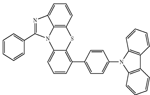
[Chemical Formula 2-2-43]
