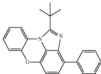
[Chemical Formula 1-11-2]
