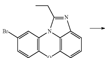
[Compound 17-D]
