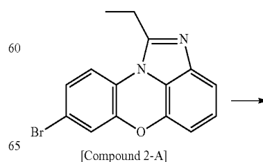
[Compound 2-A]
