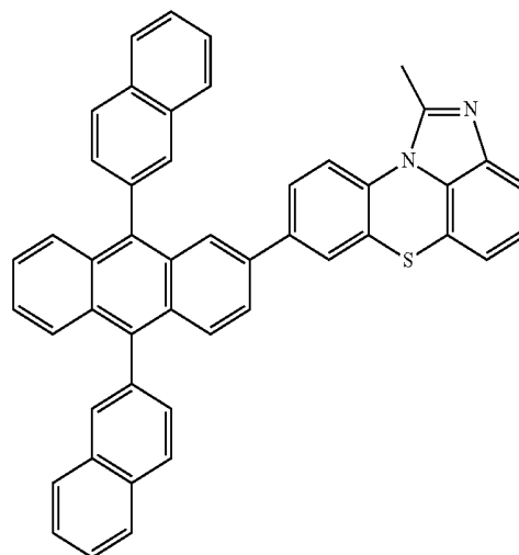
[Chemical Formula 2-2-20]
