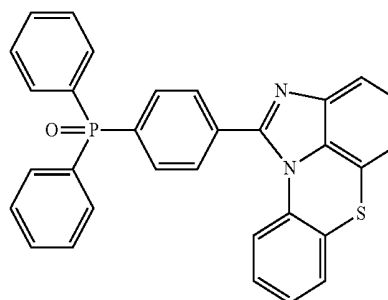
[Chemical Formula 2-1-10]
