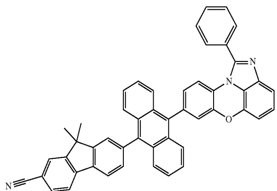
[Chemical Formula 1-4-15]
