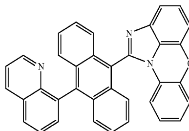
[Chemical Formula 1-1-20]
