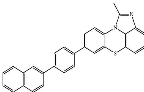
[Chemical Formula 2-2-27]
