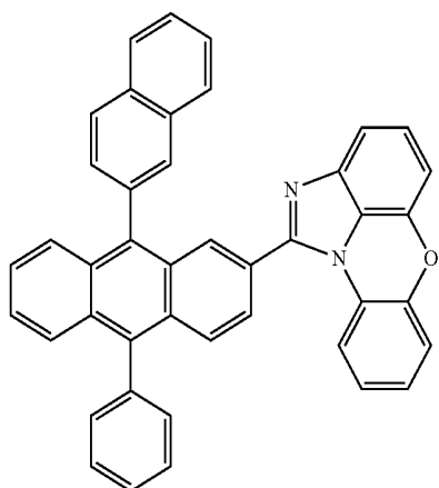
[Chemical Formula 1-1-31]
