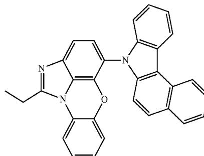
[Chemical Formula 1-9-15]
