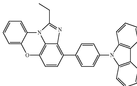
[Chemical Formula 1-11-7]
