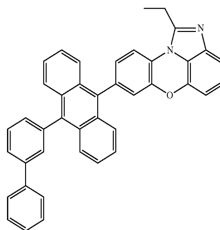
[Chemical Formula 1-3-6]
