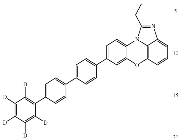
[Chemical Formula 1-3-53]
