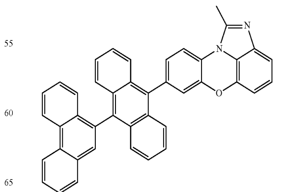
[Chemical Formula 1-2-7]
