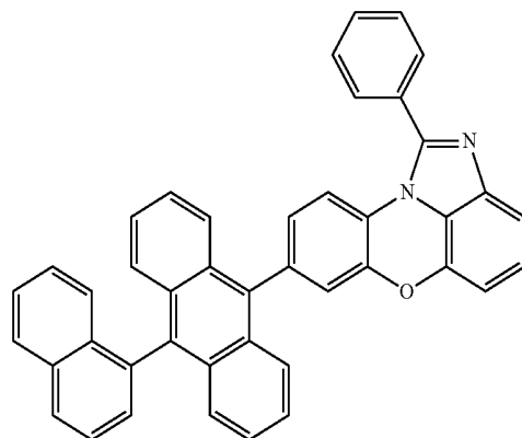
[Chemical Formula 1-4-3]
