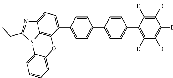
[Chemical Formula 1-9-16]
