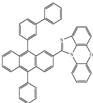
[Chemical Formula 1-1-32]
