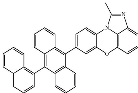
[Chemical Formula 1-2-3]
