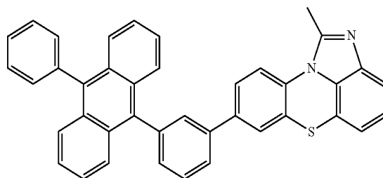
[Chemical Formula 2-2-19]
