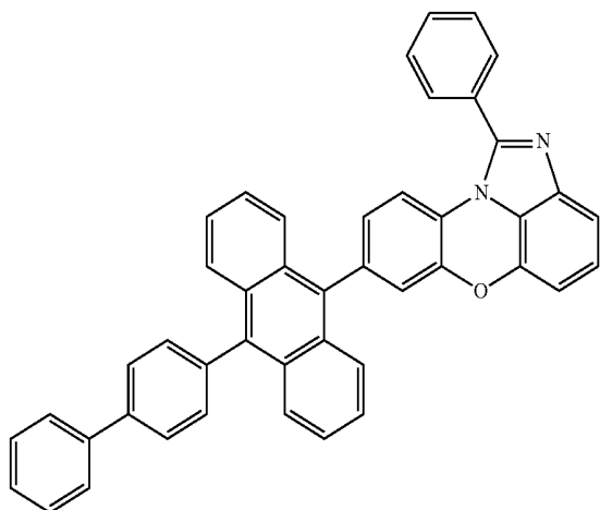
[Chemical Formula 1-4-4]
