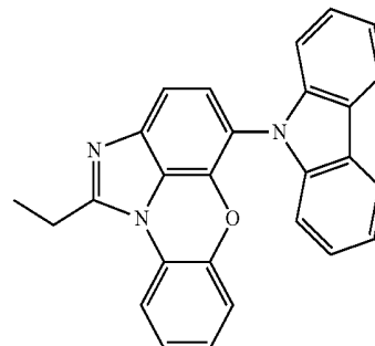
[Chemical Formula 1-9-15]
