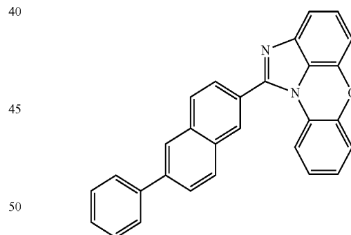
[Chemical Formula 1-1-35]
