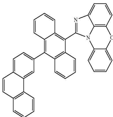
[Chemical Formula 1-1-16]
