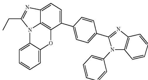
[Chemical Formula 1-9-9]
