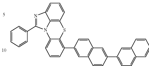
[Chemical Formula 2-2-45]
