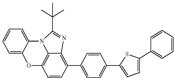
[Chemical Formula 1-11-3]
