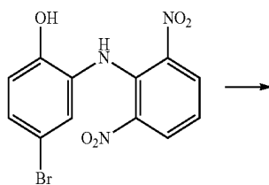
[Compound 17-A]
