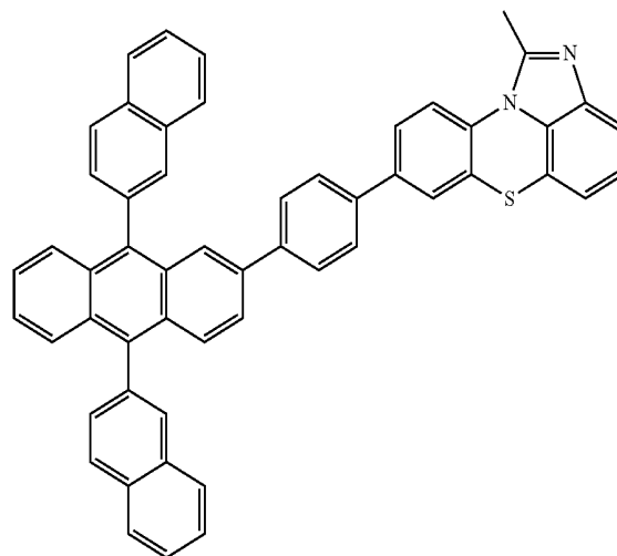
[Chemical Formula 2-2-26]
