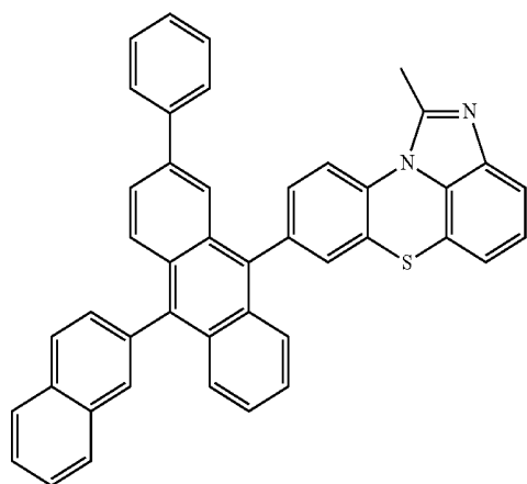
[Chemical Formula 2-2-16]
