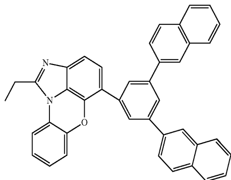
[Chemical Formula 1-9-8]
