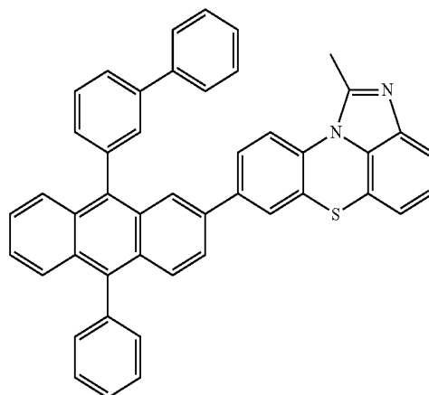
[Chemical Formula 2-2-25]
