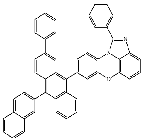
[Chemical Formula 1-4-16]
