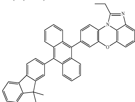
[Chemical Formula 1-3-5]
