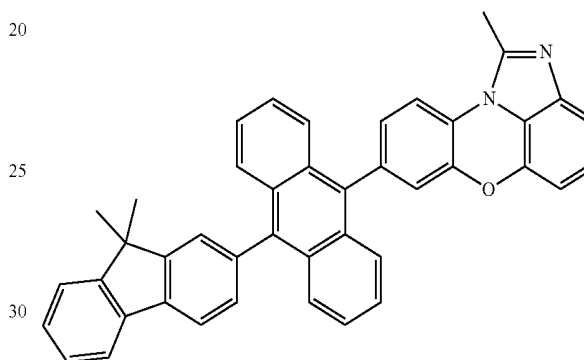
[Chemical Formula 1-2-6]
