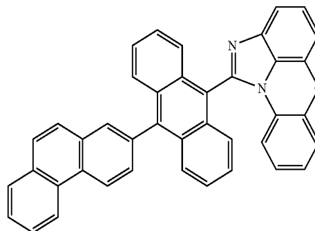
[Chemical Formula 1-1-18]
