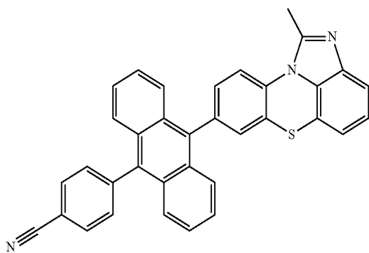
[Chemical Formula 2-2-12]
