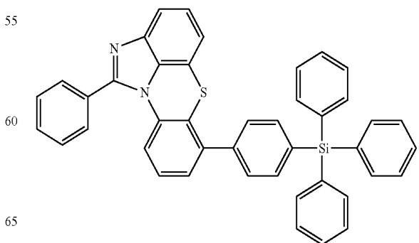
[Chemical Formula 2-2-48]
