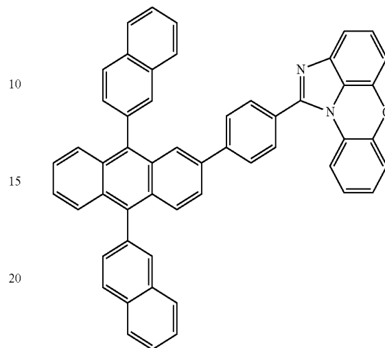
[Chemical Formula 1-1-34]
