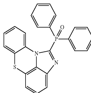
[Chemical Formula 2-1-6]
