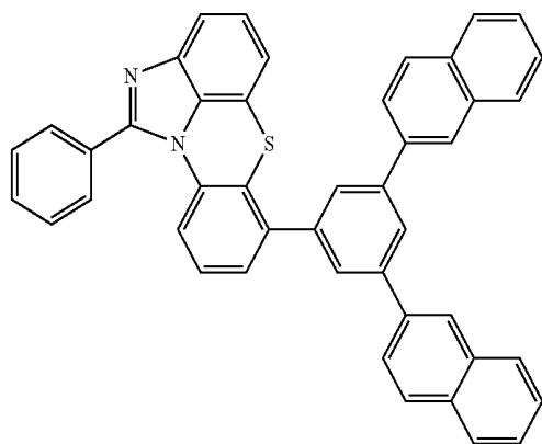
[Chemical Formula 2-2-43]
