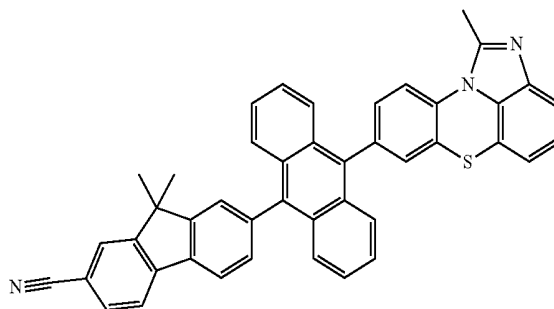
[Chemical Formula 2-2-16]
