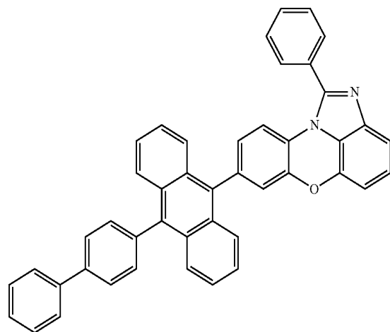
[Chemical Formula 1-4-4]
