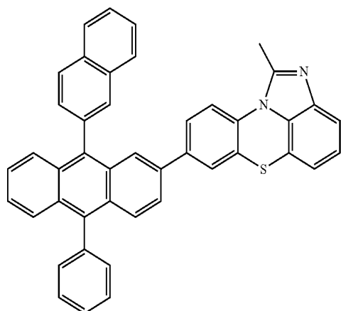
[Chemical Formula 2-2-23]
