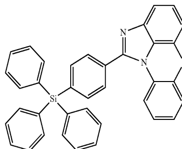
[Chemical Formula 2-1-9]
