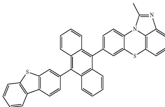
[Chemical Formula 2-2-14]
