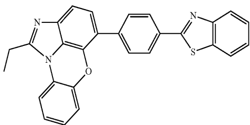
[Chemical Formula 1-9-11]
