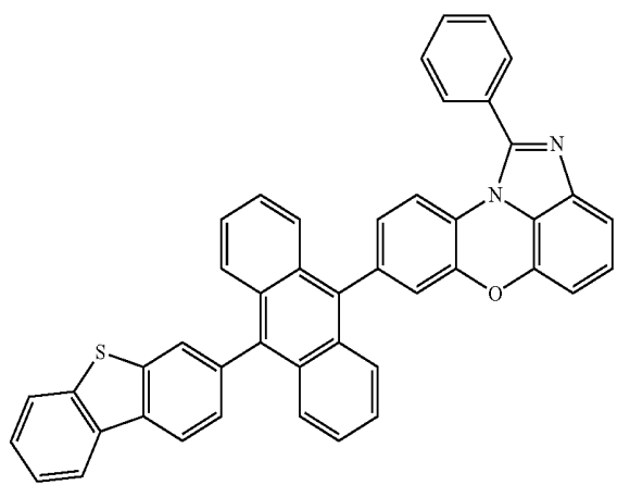
[Chemical Formula 1-4-14]
