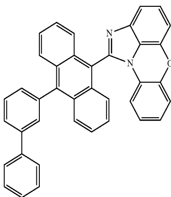
[Chemical Formula 1-1-14]
