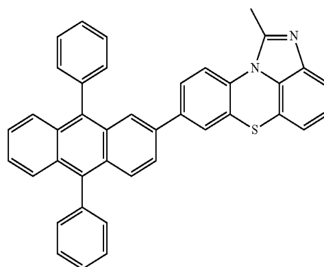
[Chemical Formula 2-2-19]
