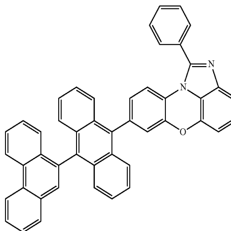
[Chemical Formula 1-4-7]
