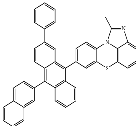
[Chemical Formula 2-2-16]
