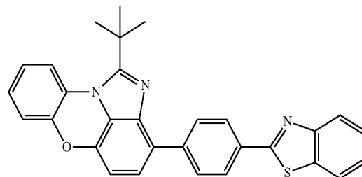
[Chemical Formula 1-11-10]
