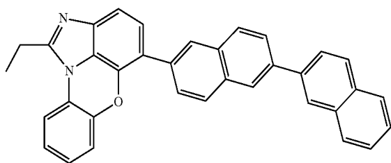
[Chemical Formula 1-9-8]
