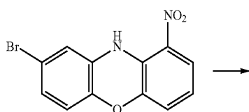
[Compound 17-B]
