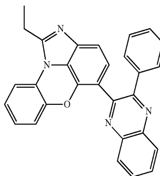
[Chemical Formula 1-9-8]
