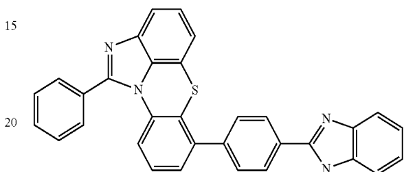
[Chemical Formula 2-2-45]
