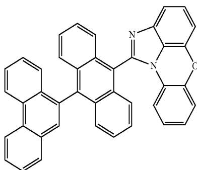
[Chemical Formula 1-1-15]
