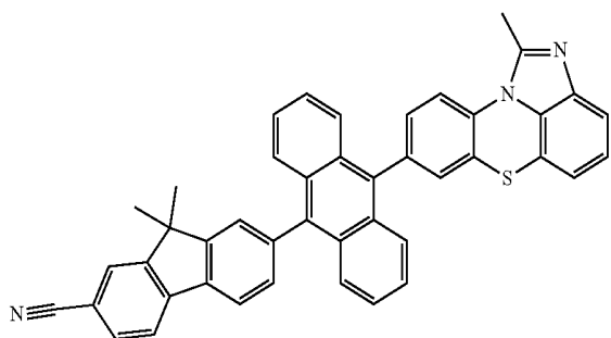
[Chemical Formula 2-2-16]
