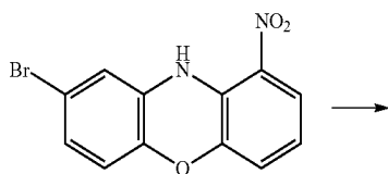
[Compound 17-C]
