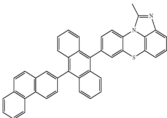
[Chemical Formula 2-2-9]
