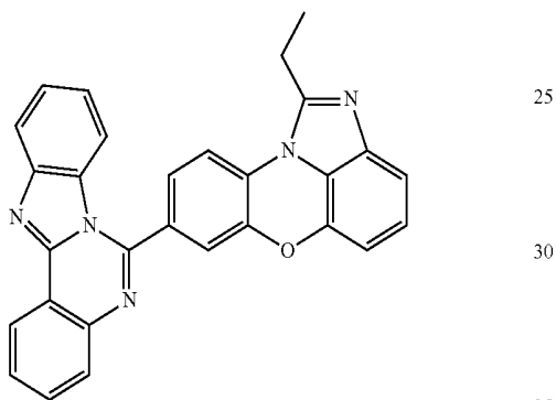
[Chemical Formula 1-3-54]
