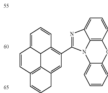
[Chemical Formula 1-1-36]
