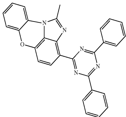
[Chemical Formula 1-11-5]
