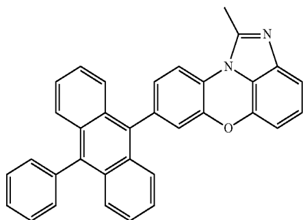
[Chemical Formula 1-2-2]
