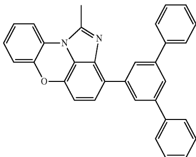
[Chemical Formula 1-11-5]
