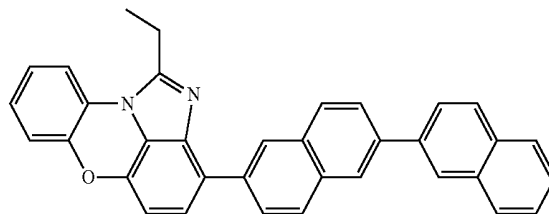
[Chemical Formula 1-11-9]
