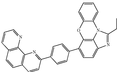
[Chemical Formula 1-9-11]
